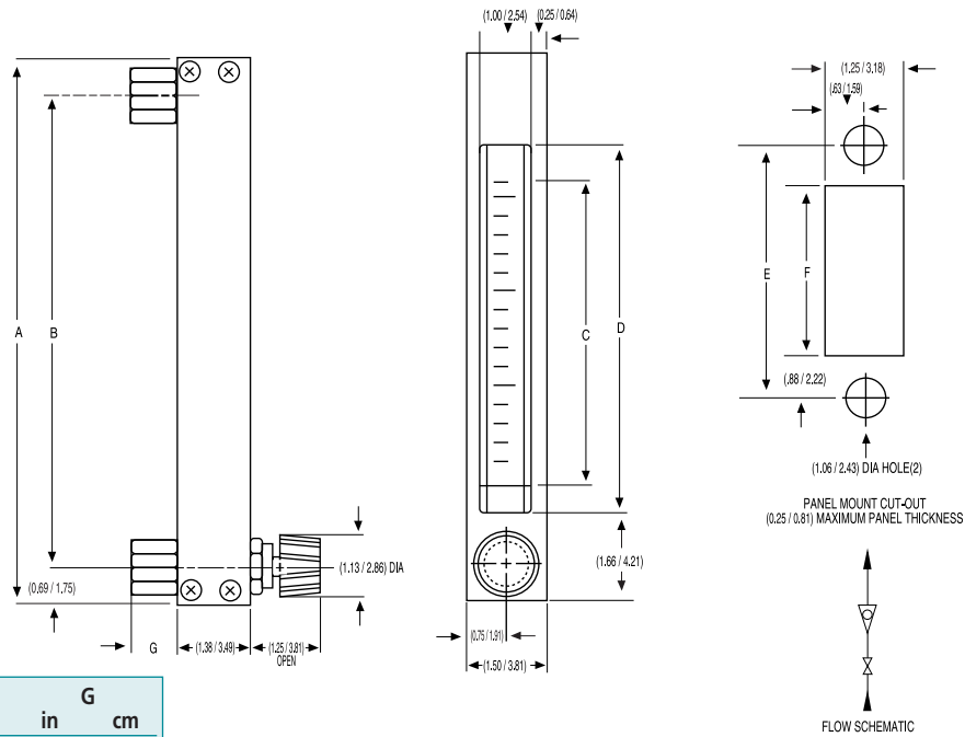
FLOW SCHEMATIC
